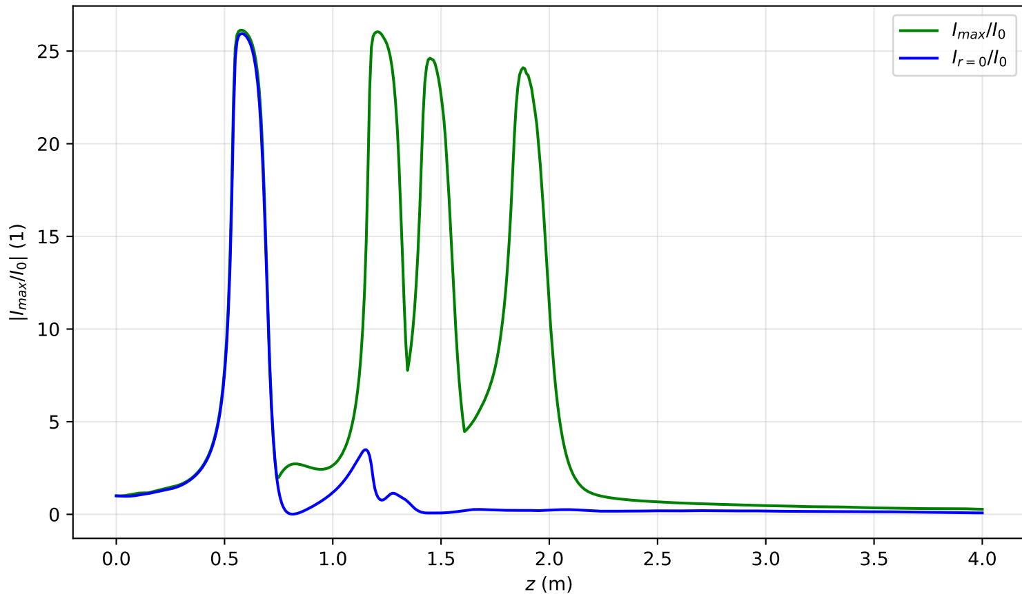
I_{max}(x=0, y=0, z)/I_0 , P_{in}=4.2P_{cr} , noisy input, artificial time
